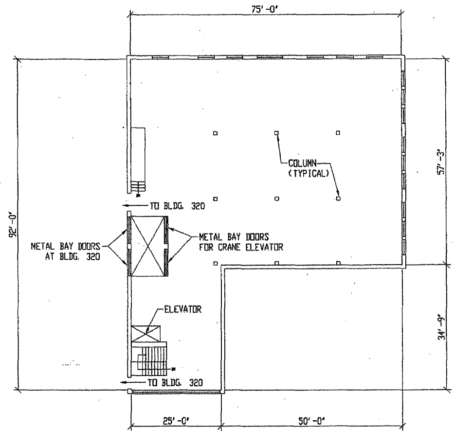
5TH FLOOR PLAN (BLDG. 322)
